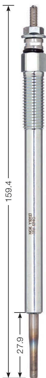
Y1012 J M 10 x 1.25 10 Hex 11 V DP 65 158
