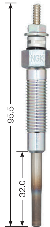
Y-118 R M 10 x 1.25 12 Hex 7 V
