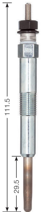
Y-749 J M 10 x 1.0 10 Hex 11 V
