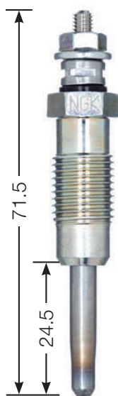
Y-928 U M 12 x 1.25 12 Hex 11 V DP 29 156
