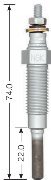
Y-116 V M 10 x 1.25 12 Hex 10.5 V
