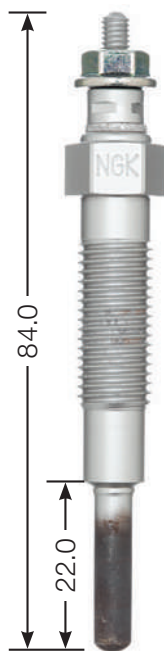
Y-110 V M 10 x 1.25 12 Hex 10.5 V
