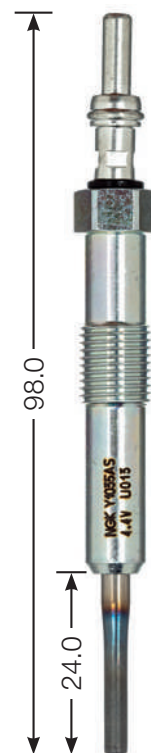
Y1035 AS M 10 x 1.0 10 Hex 4.4 V DP 77
