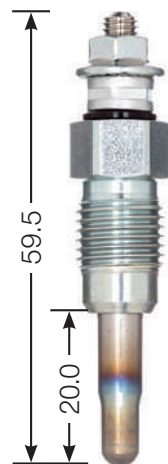
Y-918 J M 12 x 1.25 12 Hex 12 V DP 2
