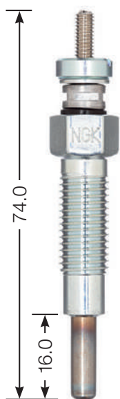
Y-106-1 M 10 x 1.25 12 Hex 10.5 V
