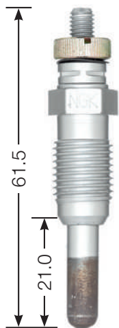
Y-204 TS1 M 12 x 1.25 12 Hex 11 V
