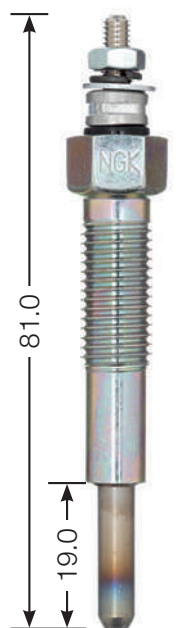
Y-771 R M 10 x 1.25 12 Hex 24 V
