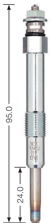
Y-747 U M 10 x 1.0 10 Hex 11 V DP 26
