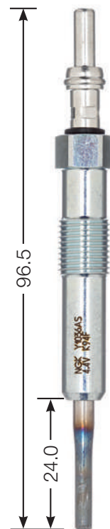
Y1036 AS M 10 x 1.0 10 Hex 4.4 V
