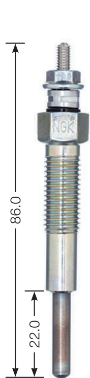
Y-107 T M 10 x 1.25 12 Hex 8.5 V
