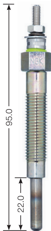
Y-115 R1 M 10 x 1.25 12 Hex 6 V
