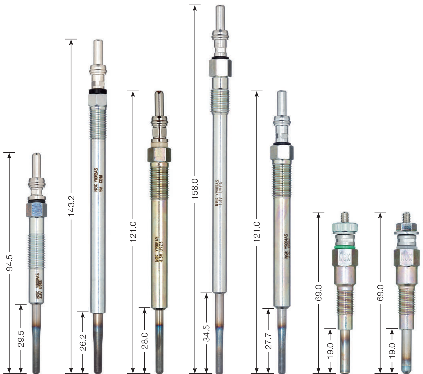
Y8009 AS M 8 x 1.0 8 Hex 4.4 V
