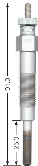
Y-117 RS M 10 x 1 12 Hex 6.5 V
