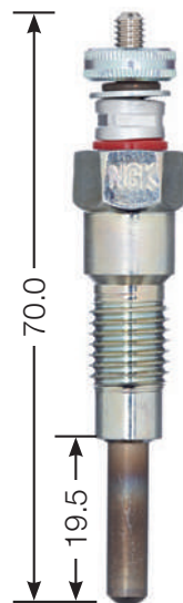
Y-112 M1 M 10 x 1.25 12 Hex 11 V
