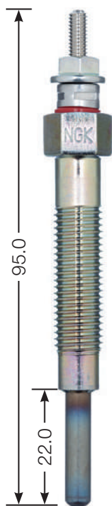
Y-115 T1 M 10 x 1.25 12 Hex 12 V
