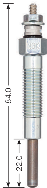
Y-110 M 10 x 1.25 12 Hex 10.5 V
