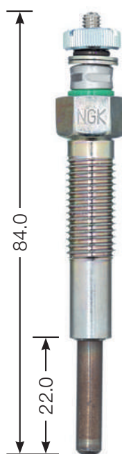
Y-107-1 M 10 x 1.25 12 Hex 10.5 V
