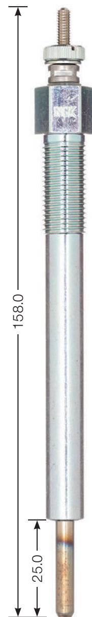
Y-203 V M 12 x 1.25 14 Hex 10.5 V
