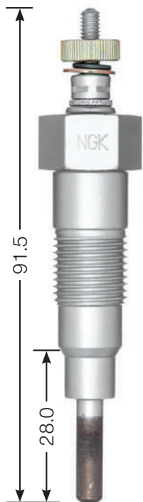
Y-402-2 M 14 x 1.25 17 Hex 8 V
